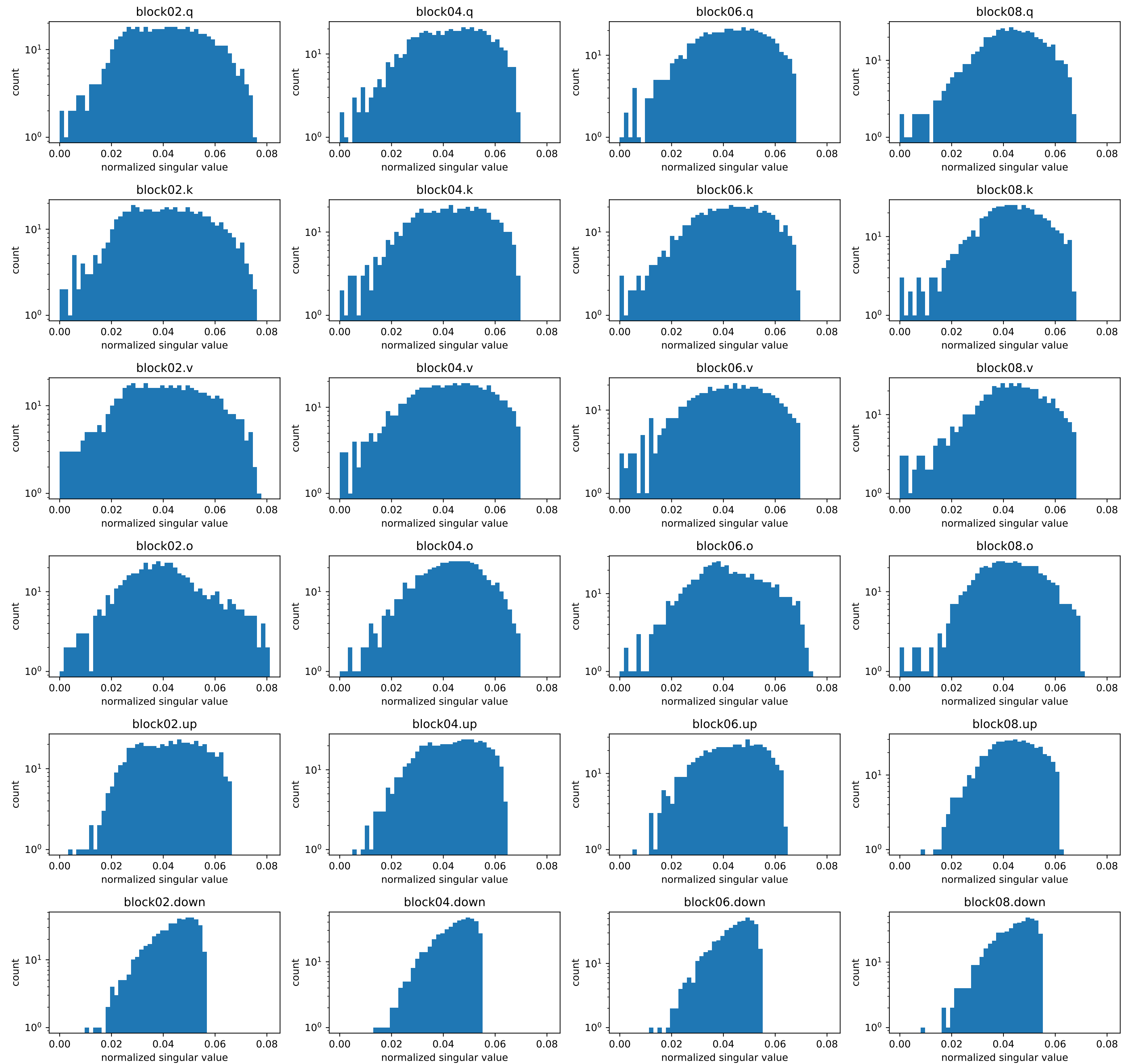
Muon post-NS update step 1469: bulk spectrum (common bins; no bulk renormalization)
