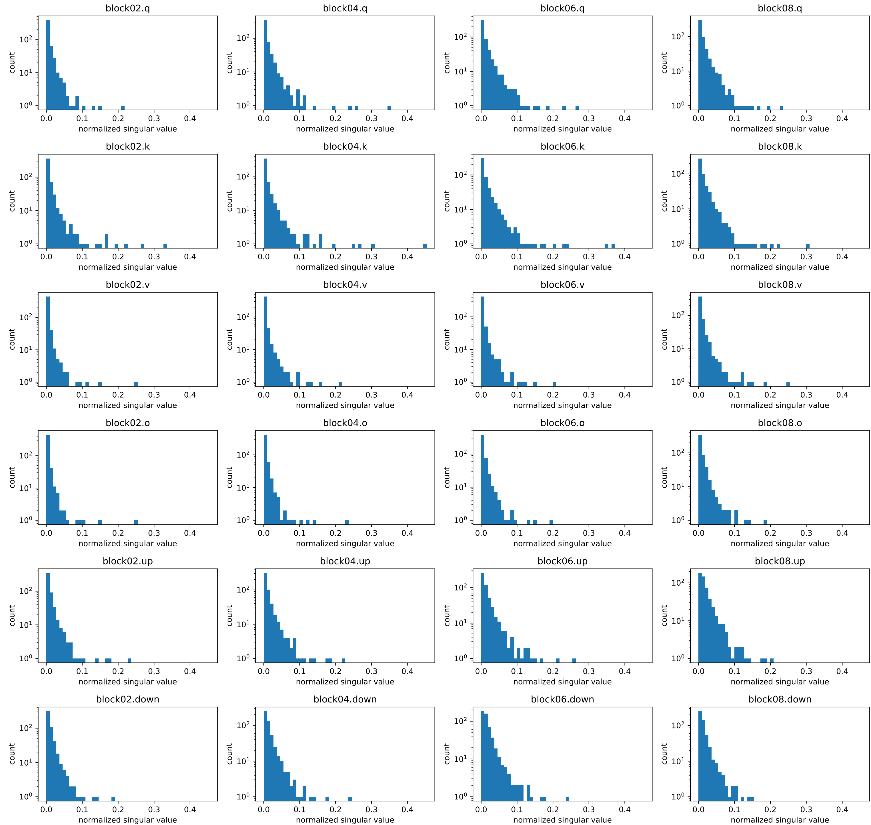
Muon pre-NS momentum step 368: bulk spectrum (common bins; no bulk renormalization)
