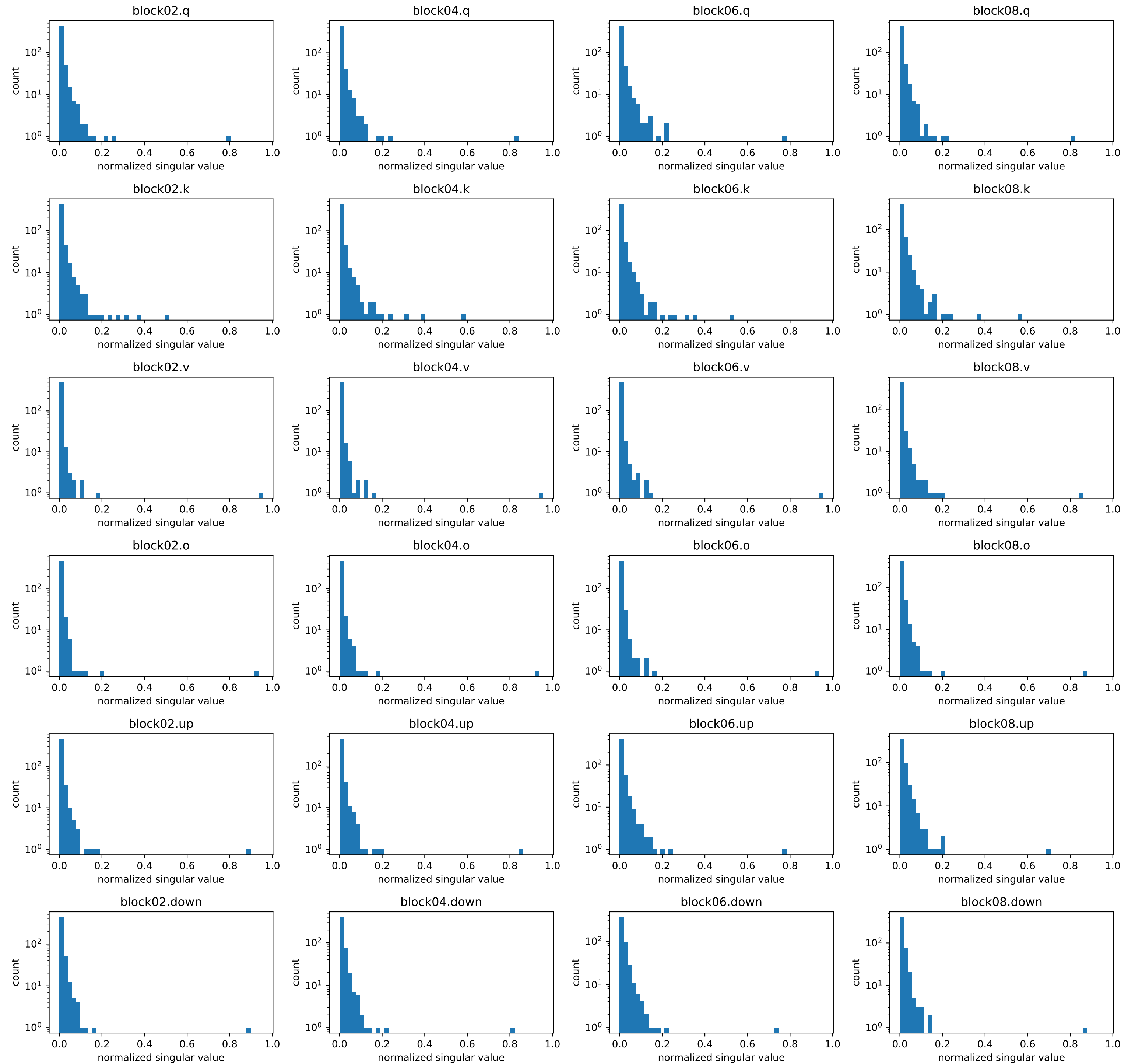
Muon pre-NS momentum step 368: full spectrum (common bins; no bulk renormalization)
