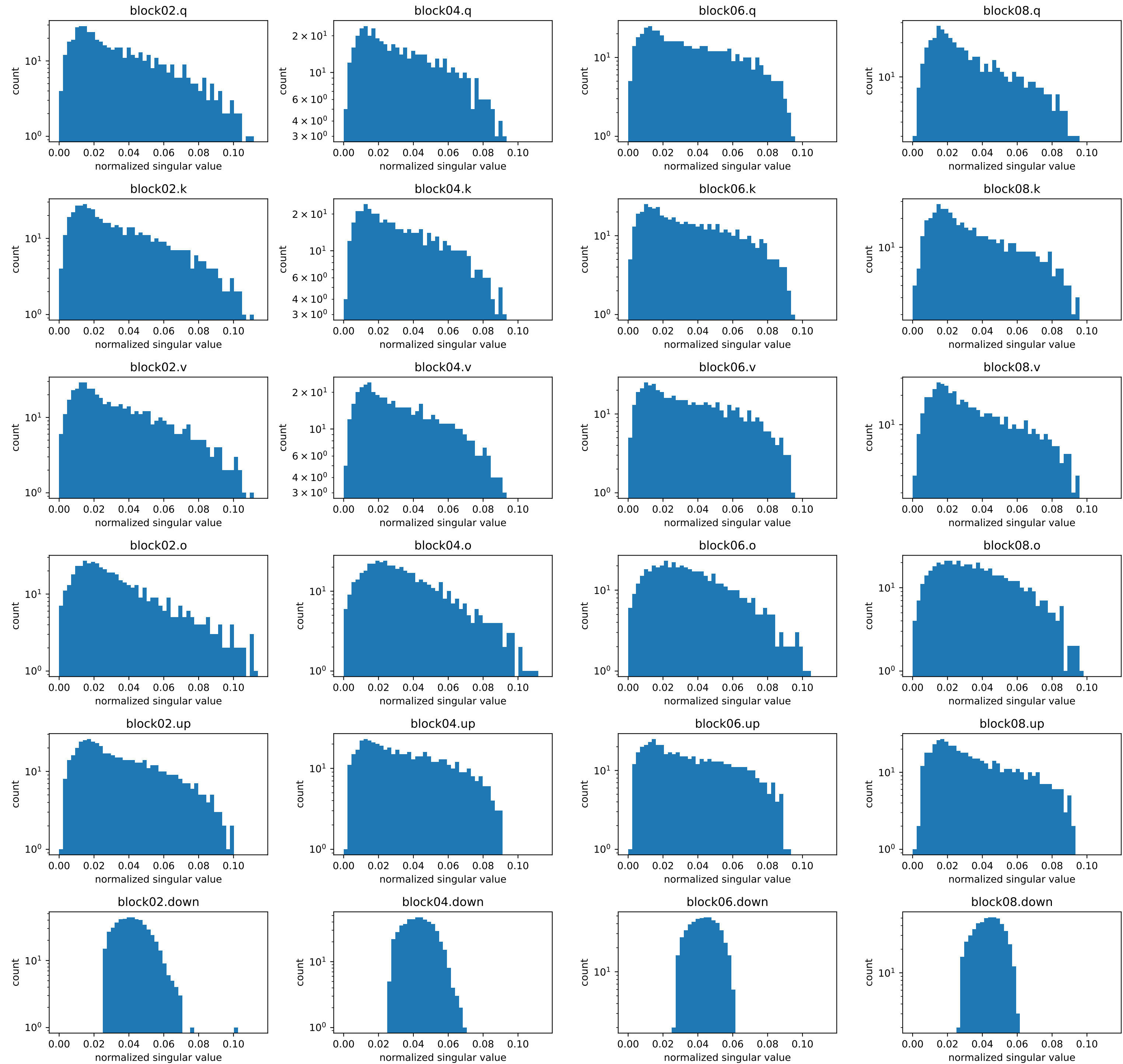
Muon post-NS update step 184: bulk spectrum (common bins; no bulk renormalization)
