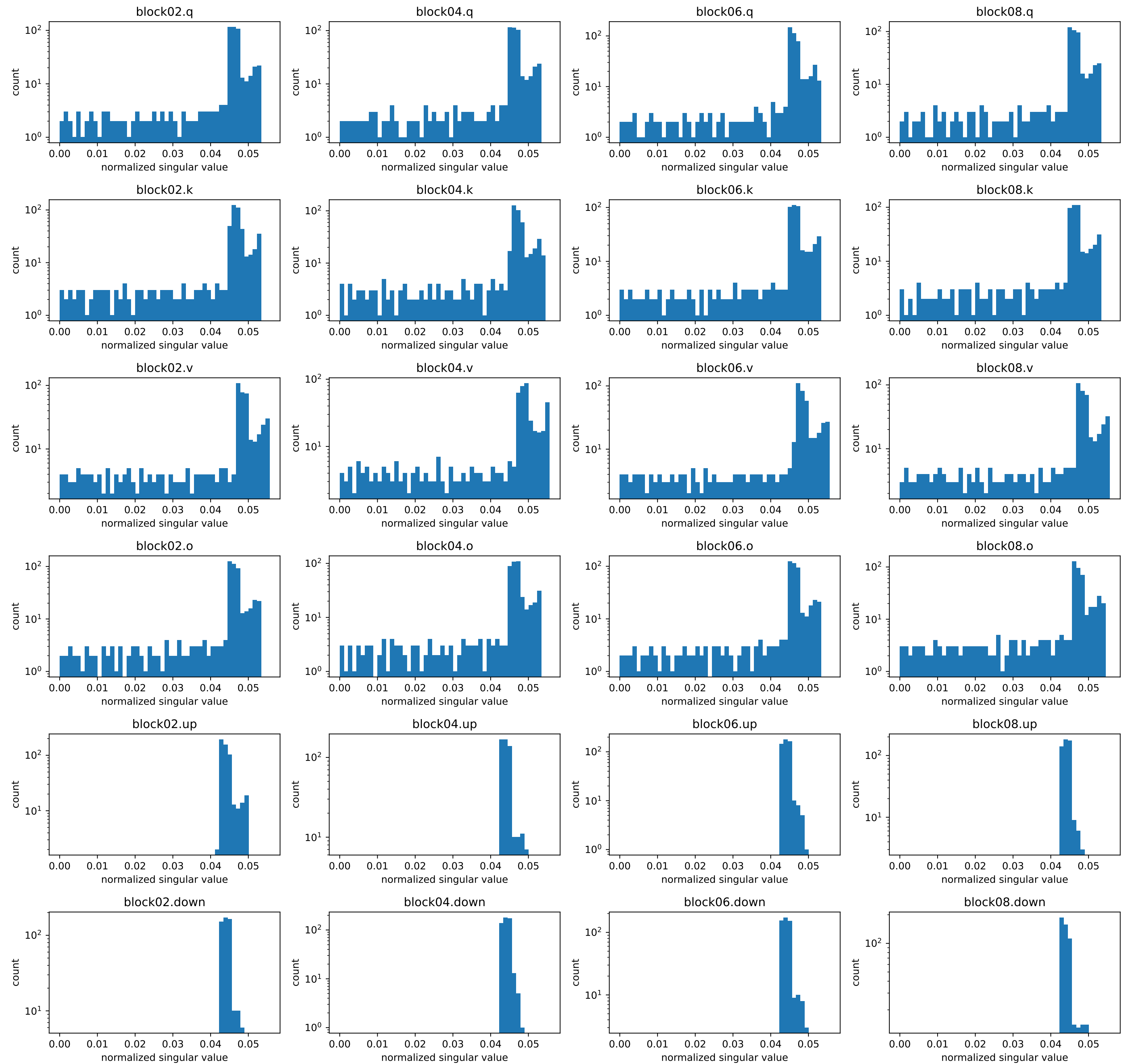
Muon post-NS update step 184: full spectrum (common bins; no bulk renormalization)
