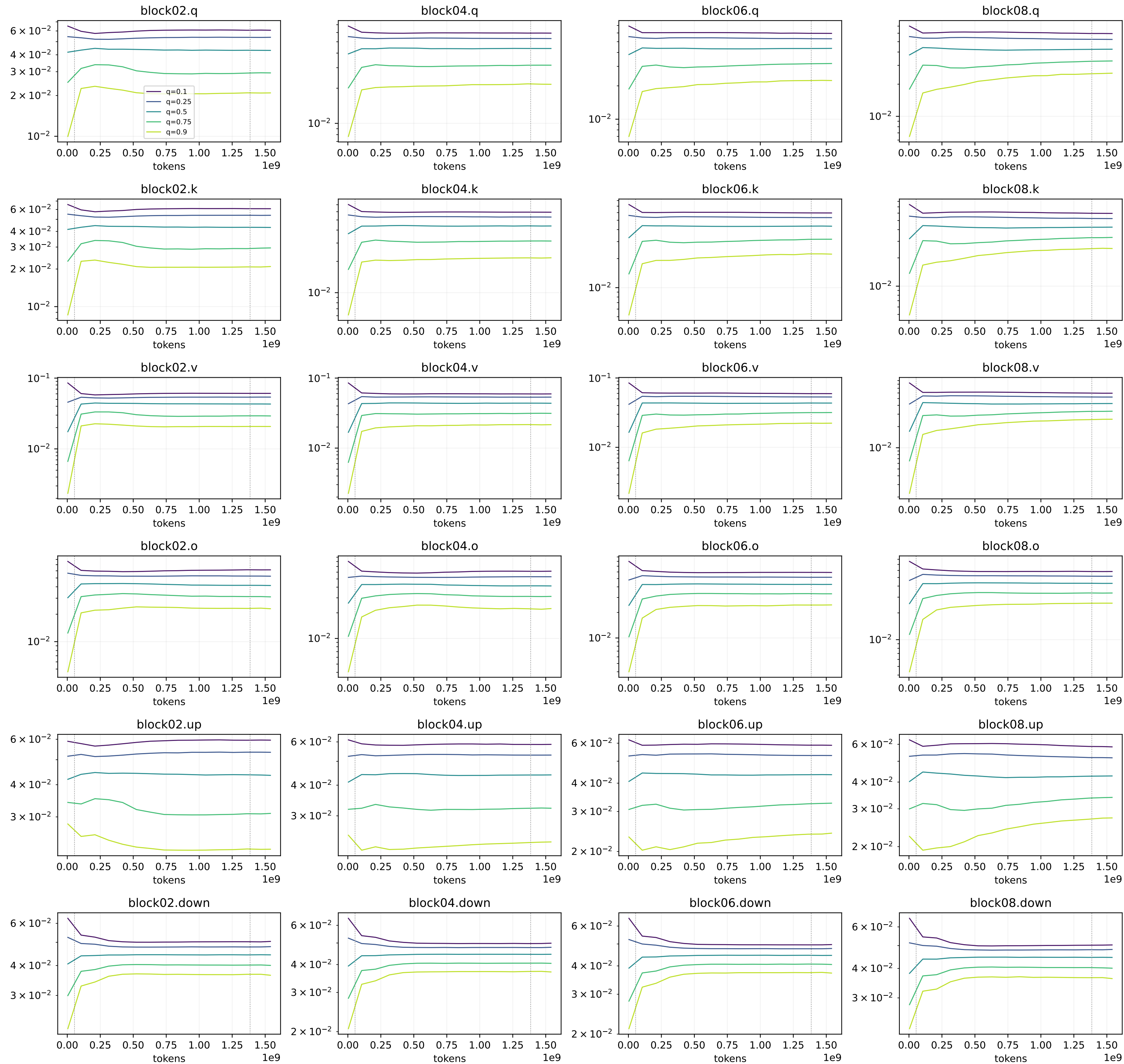
Muon post-NS update: normalized descending-rank quantiles
