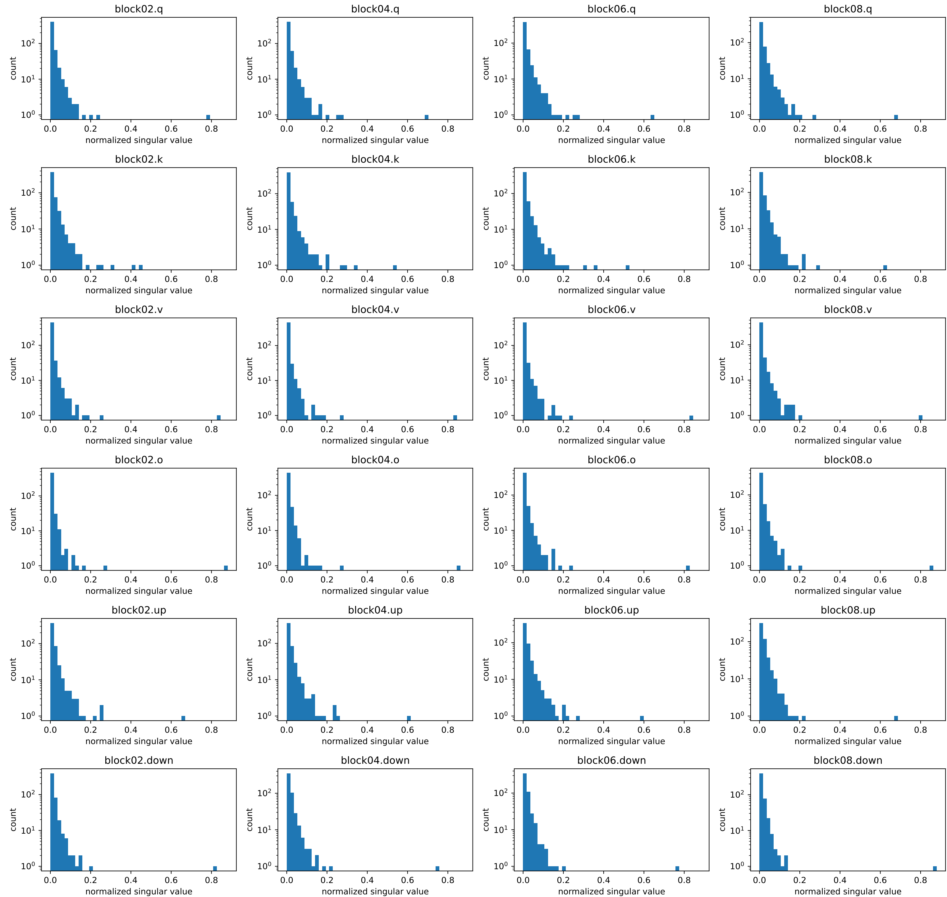
Muon pre-NS momentum step 184: full spectrum (common bins; no bulk renormalization)
