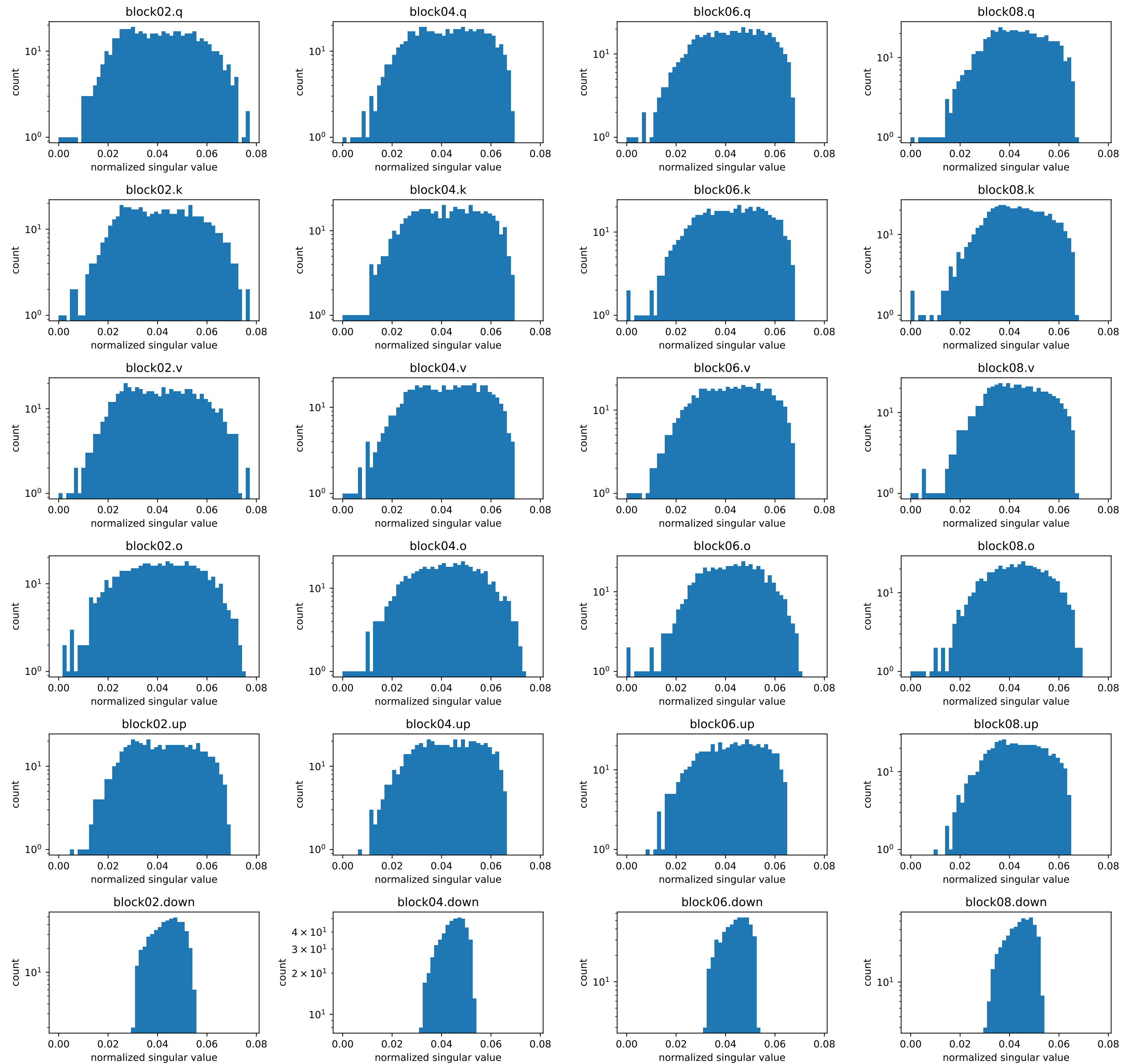
Muon post-NS update step 368: full spectrum (common bins; no bulk renormalization)
