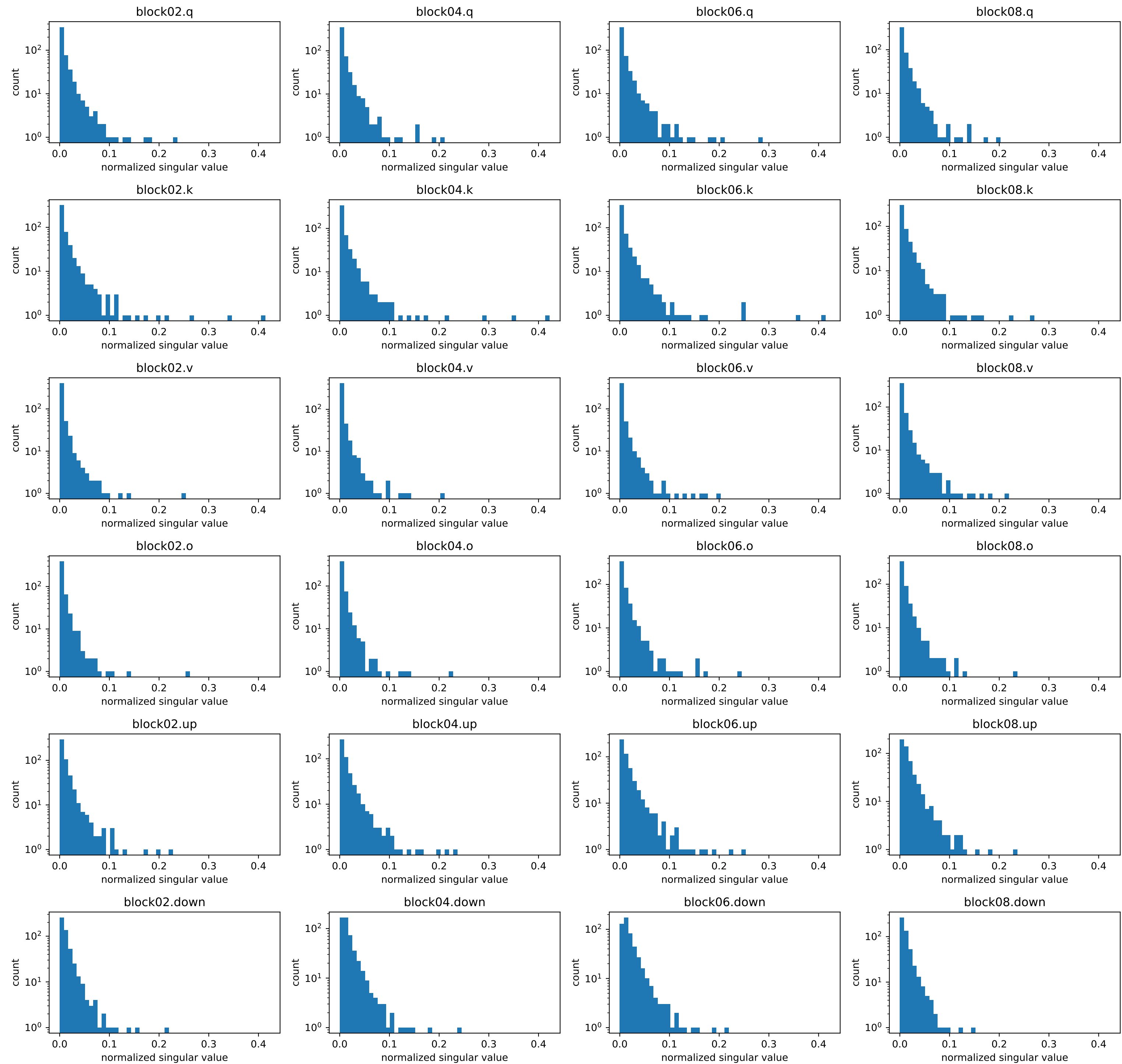
Muon pre-NS momentum step 184: bulk spectrum (common bins; no bulk renormalization)
