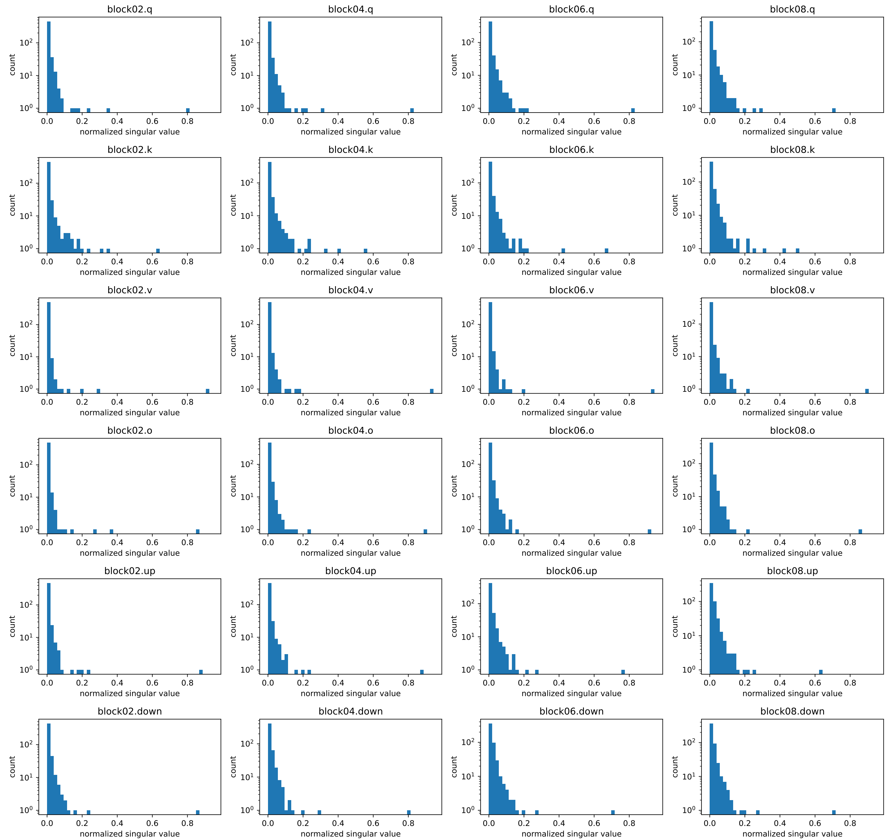
Muon pre-NS momentum step 1469: full spectrum (common bins; no bulk renormalization)
