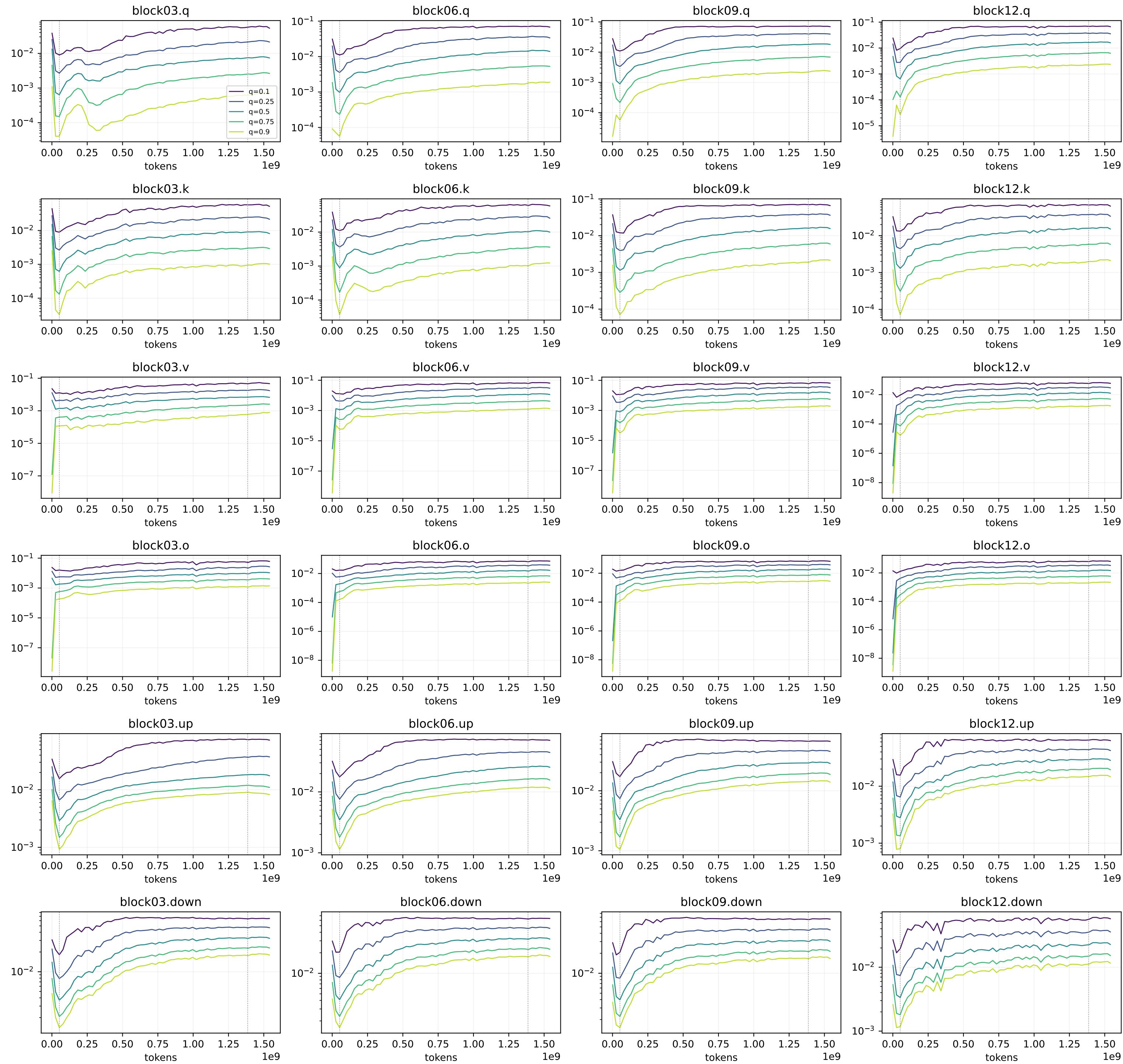
AdamW adaptive update: normalized descending-rank quantiles
