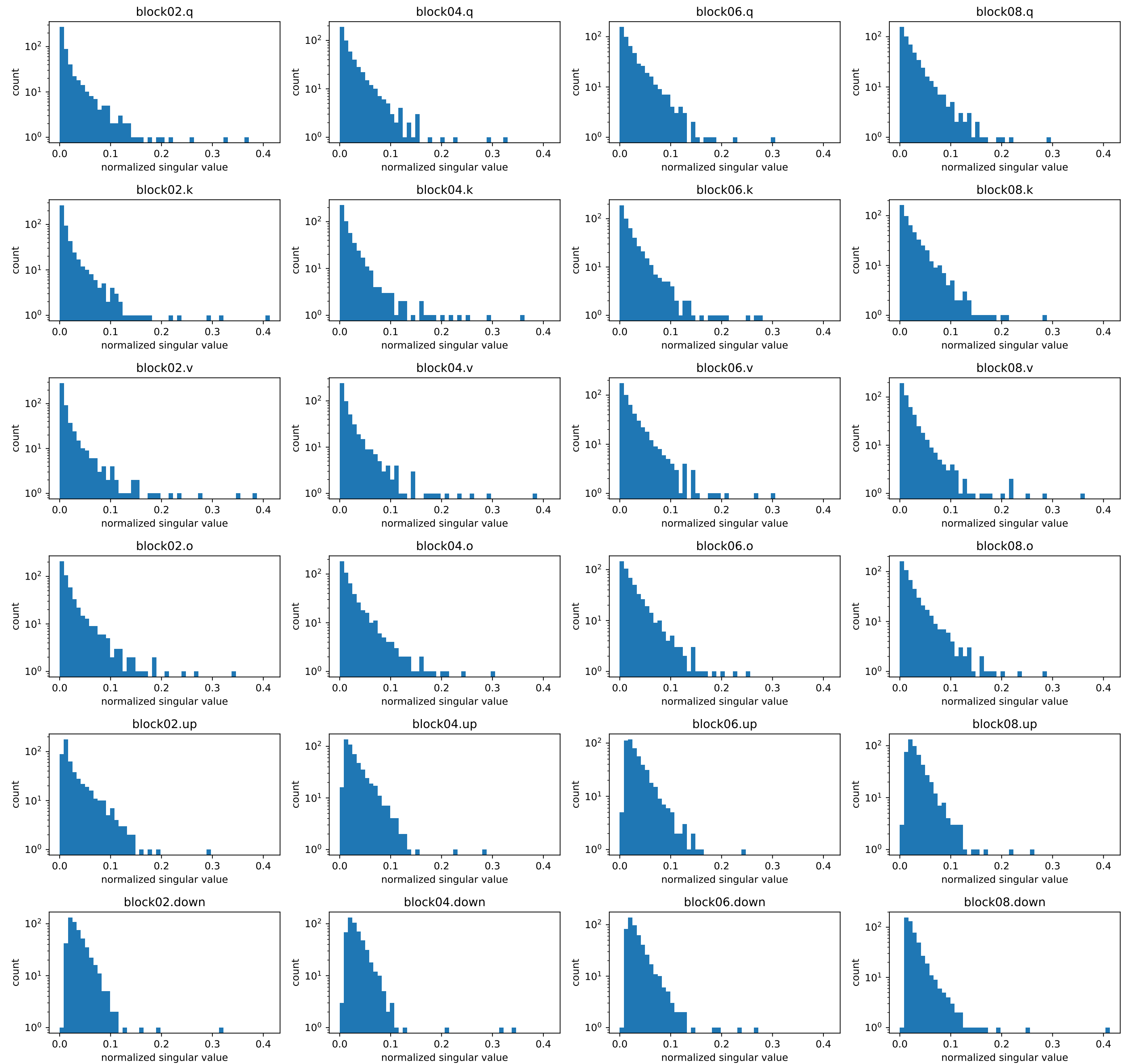
AdamW step 1469: full spectrum (common bins; no bulk renormalization)
