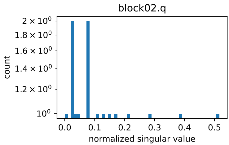
AdamW step 6: bulk spectrum (common bins; no bulk renormalization)
