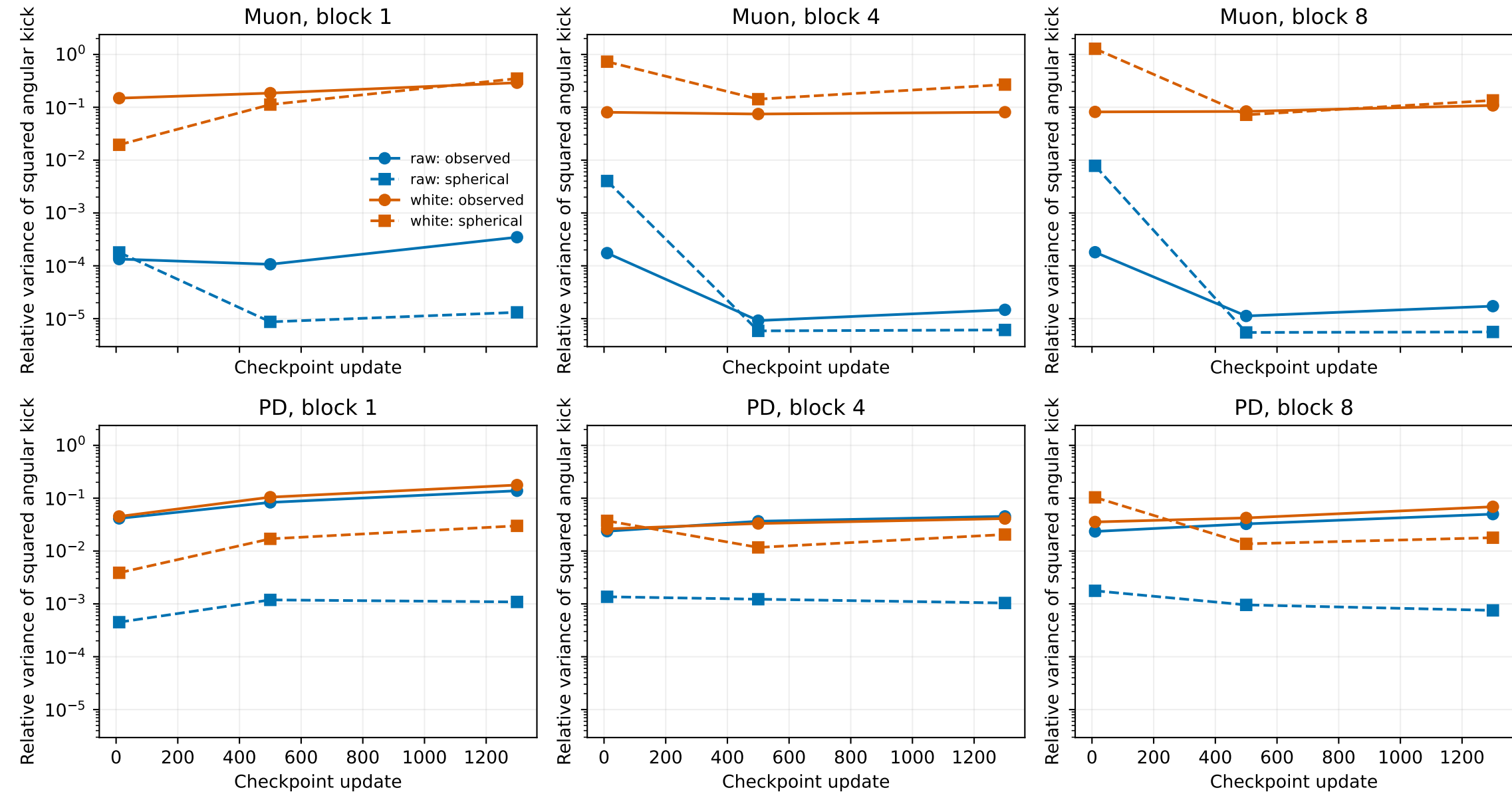
Actual-write norm dispersion: measured input directions versus spherical prediction Whitening uses regularized C; score-input lengths are normalized separately in each chart
