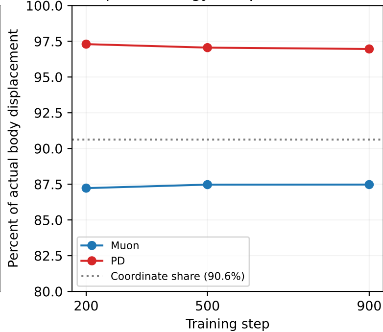
Update energy in input ranks 65+
