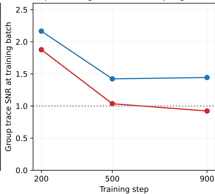
Input-tail signal versus sampling noise
