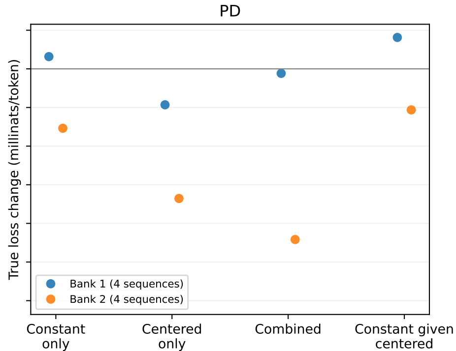
Actual value update at step500: true loss by functional component
