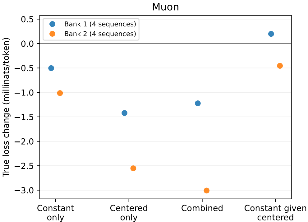
Actual value update at step500: true loss by functional component
