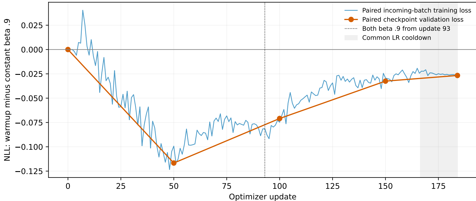
PD warmup transfer at 16M batch, doubled horizon, one matched seed
