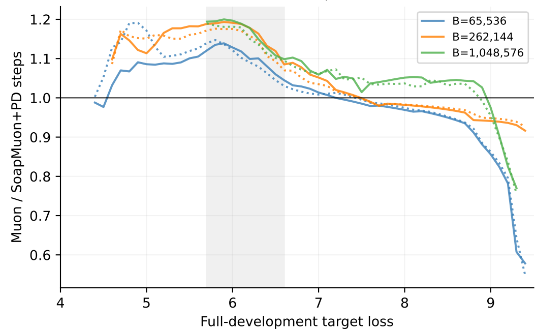
All defined thresholds, Muon LR 0.02
