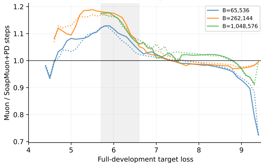
All defined thresholds, Muon LR 0.01
