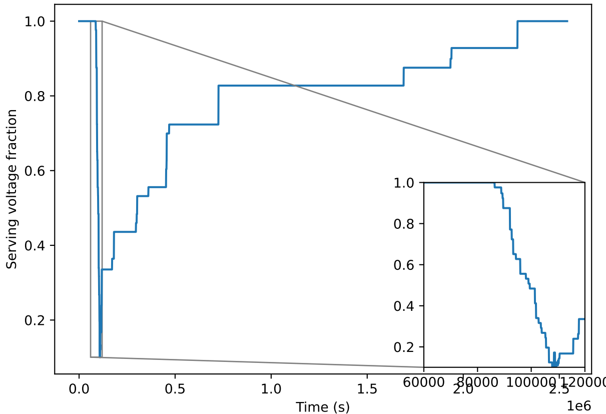
Rebound scenario voltage over time
