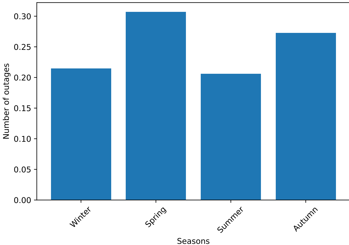
Season effect on outages
