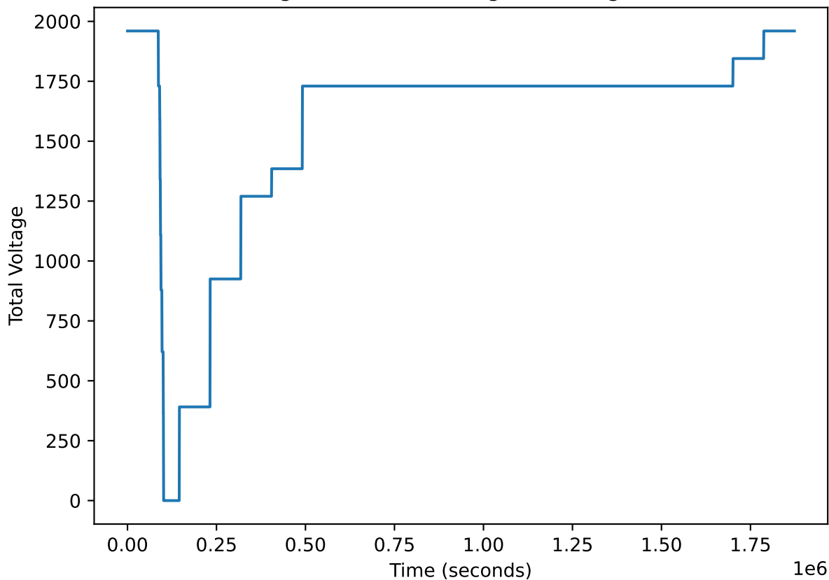
Voltage over time during cascading failure
