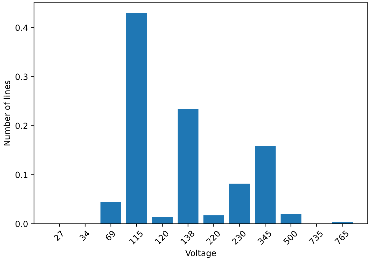
Line voltages
