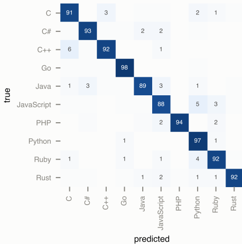
(a) Rosetta test · acc 92.7%
