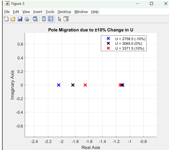
(a) Pole migration
