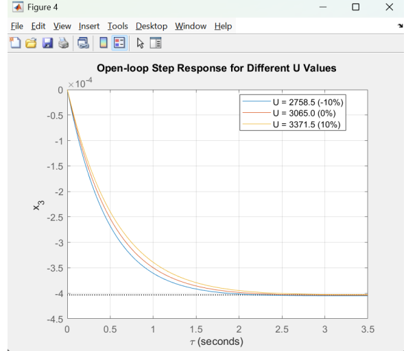
(b) Step response comparison
