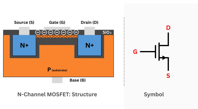
Figure 1.1: Cross-sectional structure of an N-channel MOSFET showing the inversion layer channel (left) and its corresponding schematic symbol (right).
