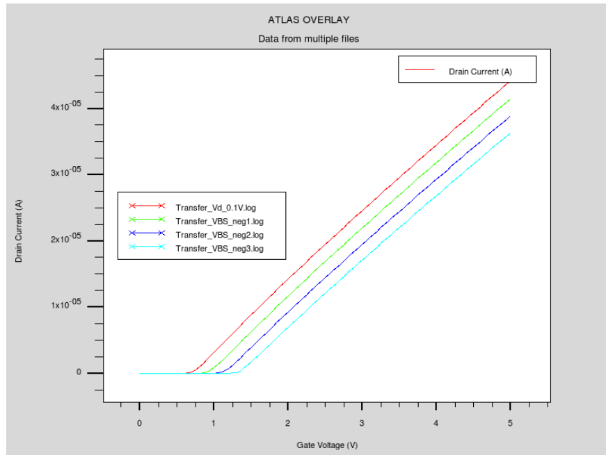
Figure 2.5: Linear-scale transfer characteristics ( I_D (A) vs. V_{GS} (V)) illustrating the body effect at V_{DS} = 0.1 V: V_{BS} = 0 V (red), -1 V (green), -2 V (blue), -3 V (cyan). The rightward shift of the curves with increasing reverse bias confirms threshold voltage enhancement.
