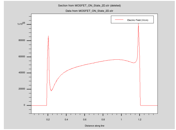
Figure 2.12: Lateral electric field |E_x| (V/cm) vs. x ( \mu\text{m} ) in the ON state ( V_{GS} = 2.0 V, V_{DS} = 1.0 V). A continuous drift field rises across the channel, peaking near the drain junction ( x \approx 1.2 \mu\text{m} ) where velocity saturation effects become relevant.
