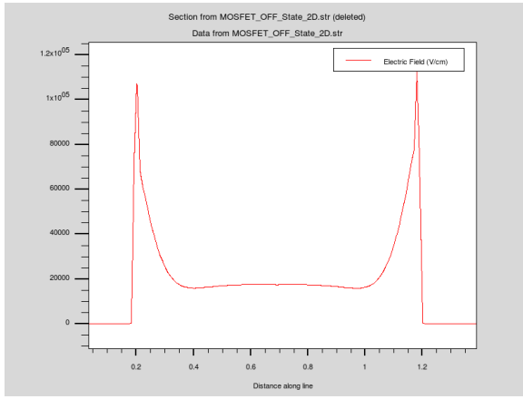
Figure 2.11: Lateral electric field |E_x| (V/cm) vs. x ( \mu\text{m} ) in the OFF state ( V_{GS} = 0 V, V_{DS} = 0.1 V). Junction field peaks at x = 0.2 and 1.2 \mu\text{m} ; the mid-channel field is low, providing no drift acceleration.
