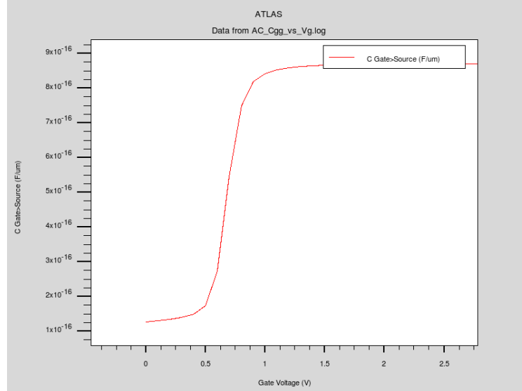
Figure 2.14: Gate-to-source capacitance C_{gs} (F/ \mu\text{m} ) vs. gate voltage V_{GS} (V), extracted from AC small-signal simulation at f = 1 MHz, V_{DS} = 0.1 V, V_{BS} = 0 V. The transition from the depletion floor ( C_{gs} \approx 1.3 \times 10^{-16} F/ \mu\text{m} ) to the strong inversion plateau ( C_{gs} \approx 8.6 \times 10^{-16} F/ \mu\text{m} ) occurs near V_{th} \approx 0.676 V.
