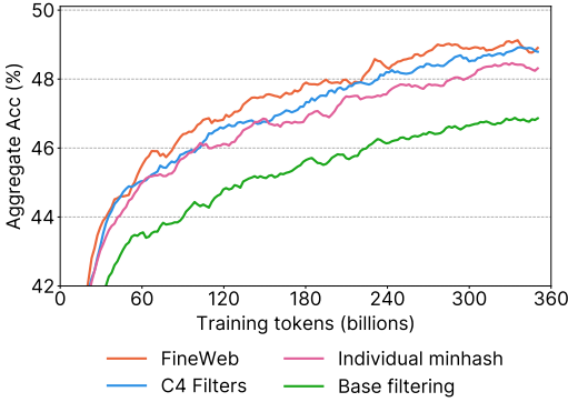
Figure 9: Each processing step in FineWeb provides a performance uplift. Compared to the base filtering (Section 3.3), applying individual-crawl Min-Hash deduplication (Section 3.4) the C4 filters (Section 3.5), and our additional heuristic filters (Section 3.6) each improve performance.
