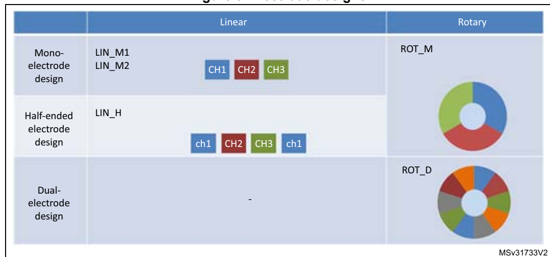
Figure 8. Electrode designs
