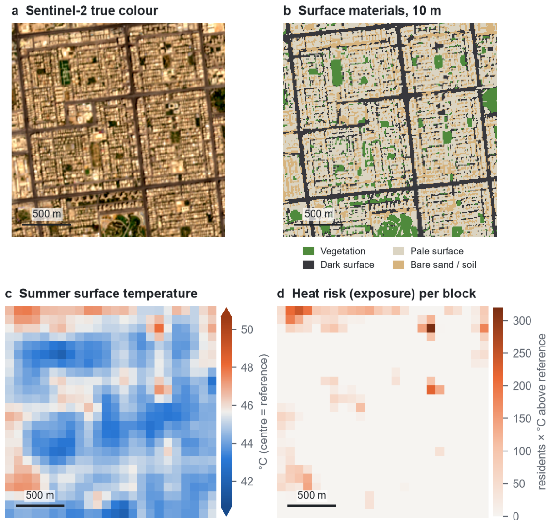
Figure 3. Nasr City display district. (a) Sentinel-2 true colour; (b) interim material classes; (c) block LST; (d) heat exposure per block, residents × °C above the reference. White blocks in (d) are cooler than the reference.
