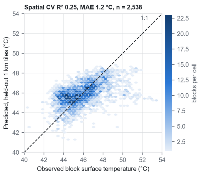
Figure 2. Observed block LST against predictions for blocks in held-out 1 km tiles.
