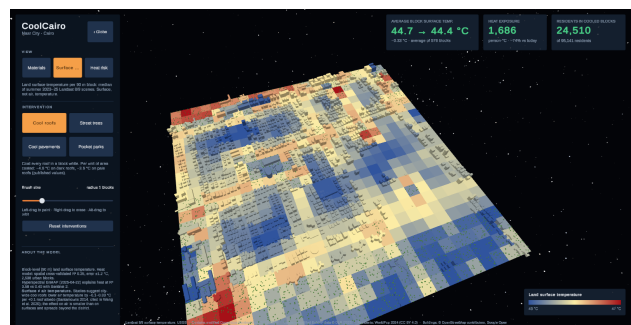
h Surface heat after the same plan.
