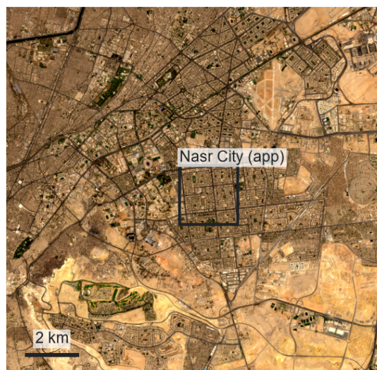
Figure 1. Model area. (a) Sentinel-2 summer median true colour; (b) Landsat summer median land surface temperature per 90 m block, centred on the urban median. Desert and bare ground (orange) are hotter than the built and irrigated city (blue). The box marks the district shown in the app.
