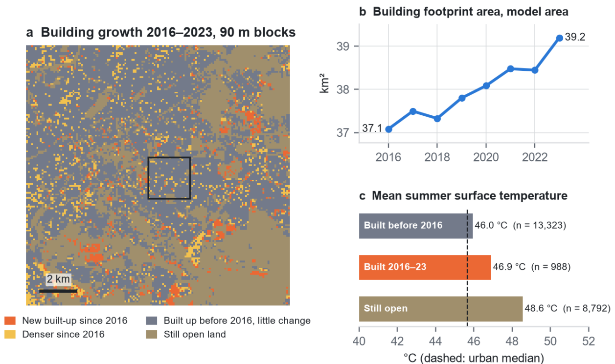
Figure 6. Urban growth 2016–2023 from Google Open Buildings Temporal. (a) Block classes, same colours as the app's Growth view; the box marks Nasr City. (b) Building footprint area per year. (c) Mean summer LST (2023–25) by class, with block counts.
