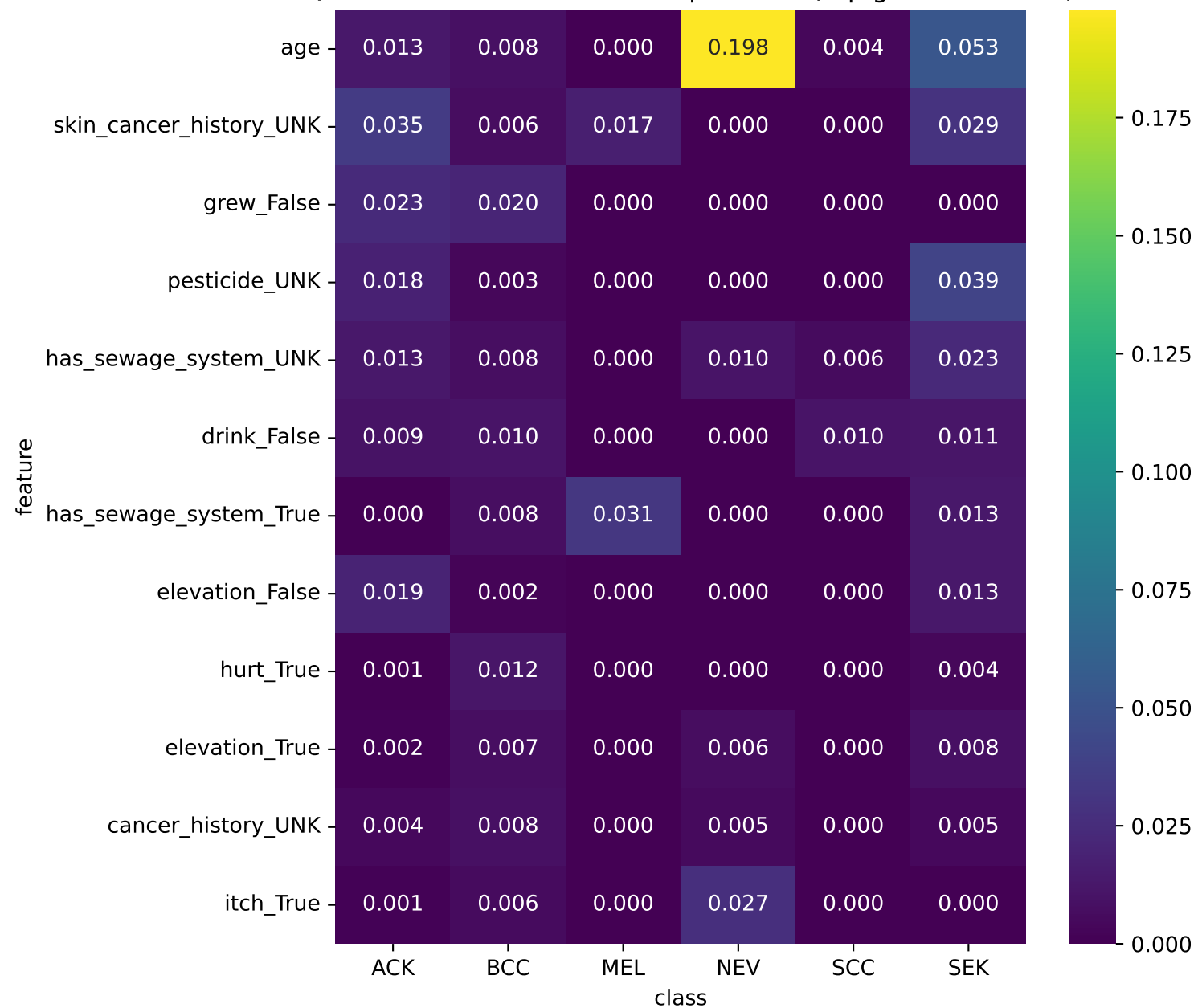
RQ2: Per-class SHAP feature importance (top global features)
