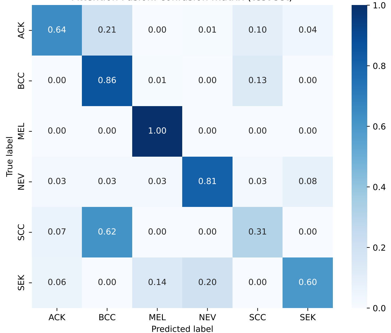
Attention Fusion: confusion matrix (test set)
