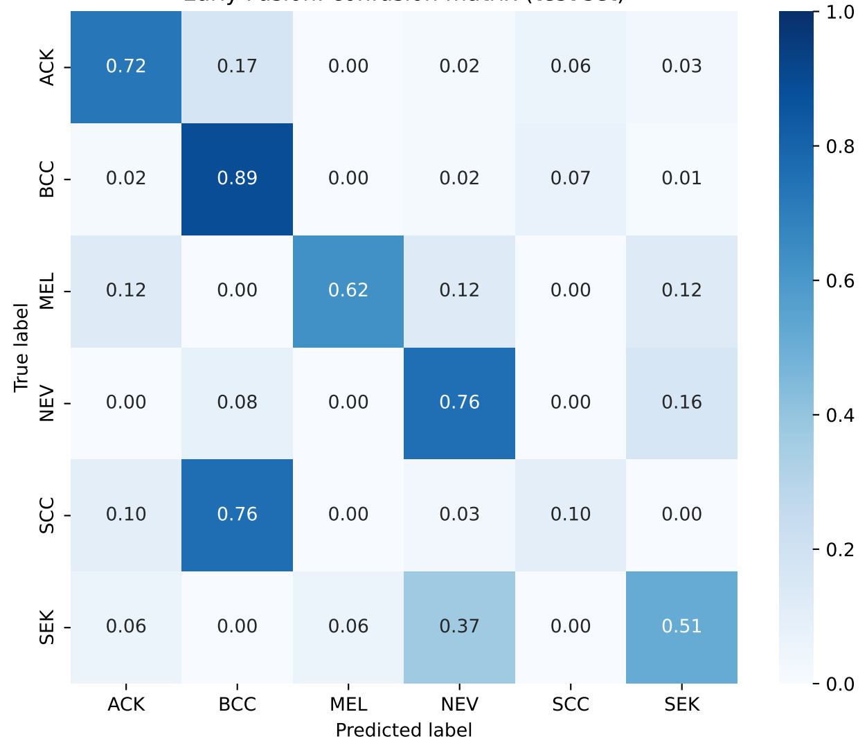
Early Fusion: confusion matrix (test set)
