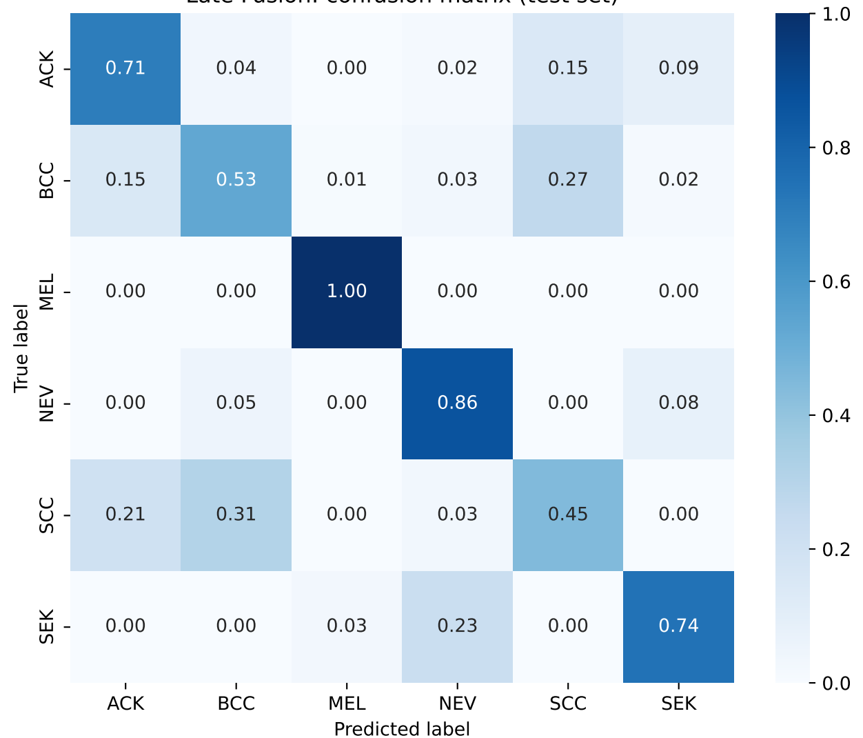
Late Fusion: confusion matrix (test set)
