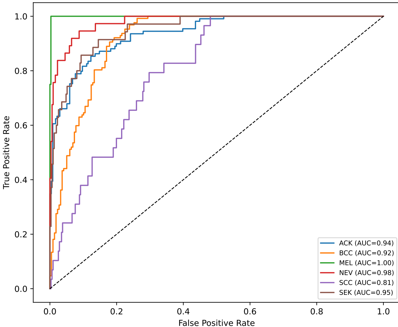
Attention Fusion: ROC curves (test set)
