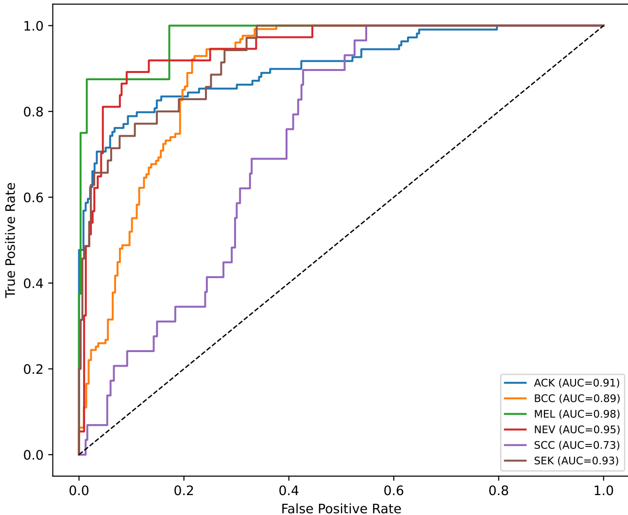
Early Fusion: ROC curves (test set)
