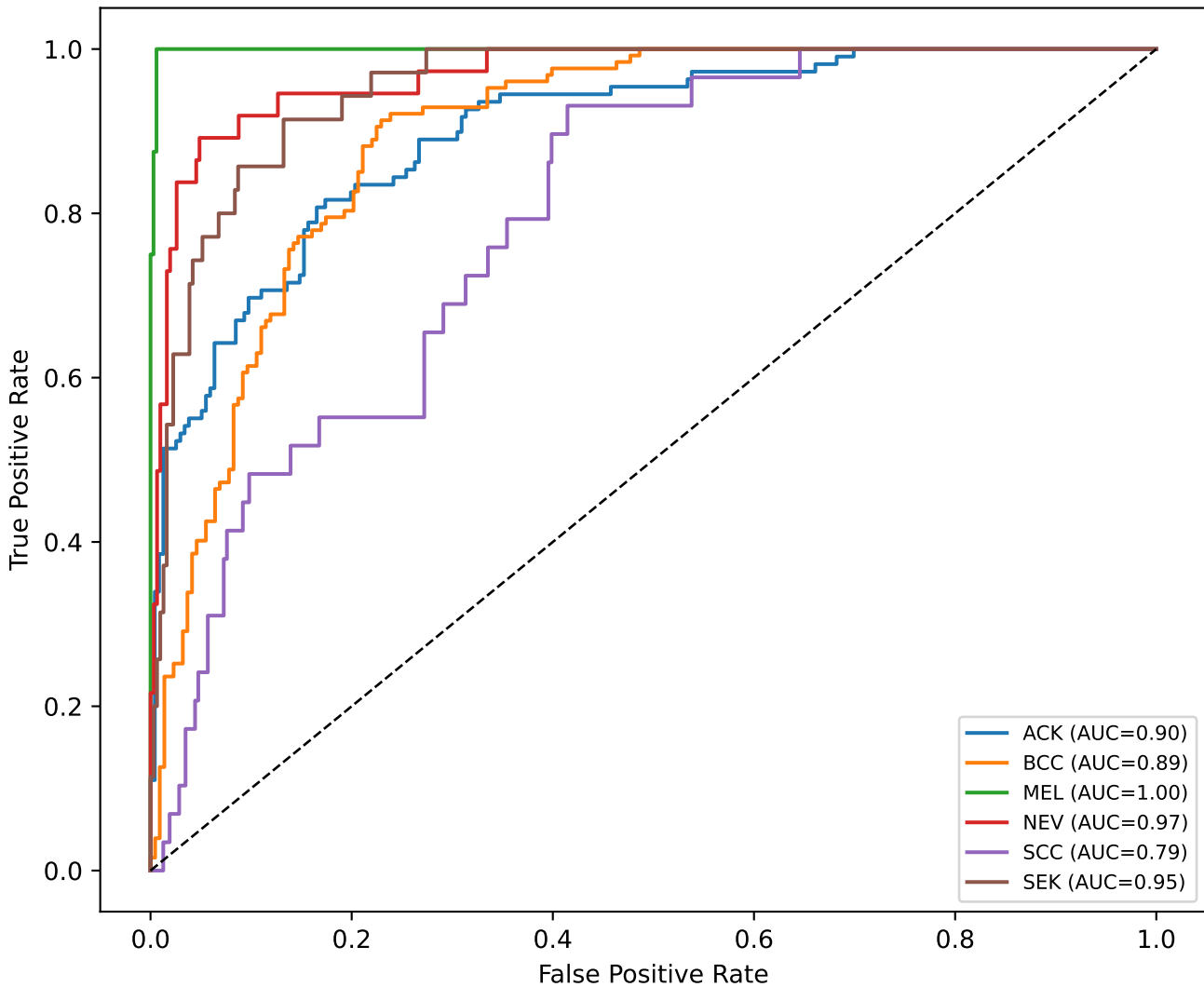
Late Fusion: ROC curves (test set)
