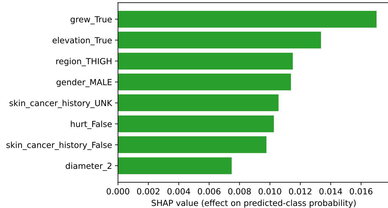
Top metadata contributions Attention weights: image=0.50, metadata=0.50
