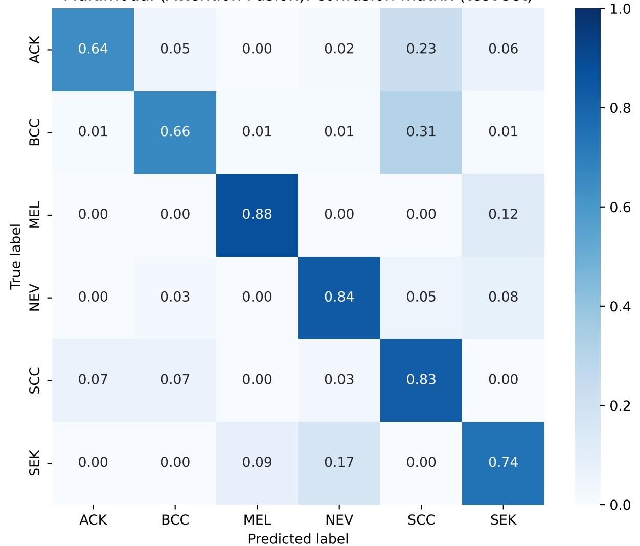
Multimodal (Attention Fusion): confusion matrix (test set)
