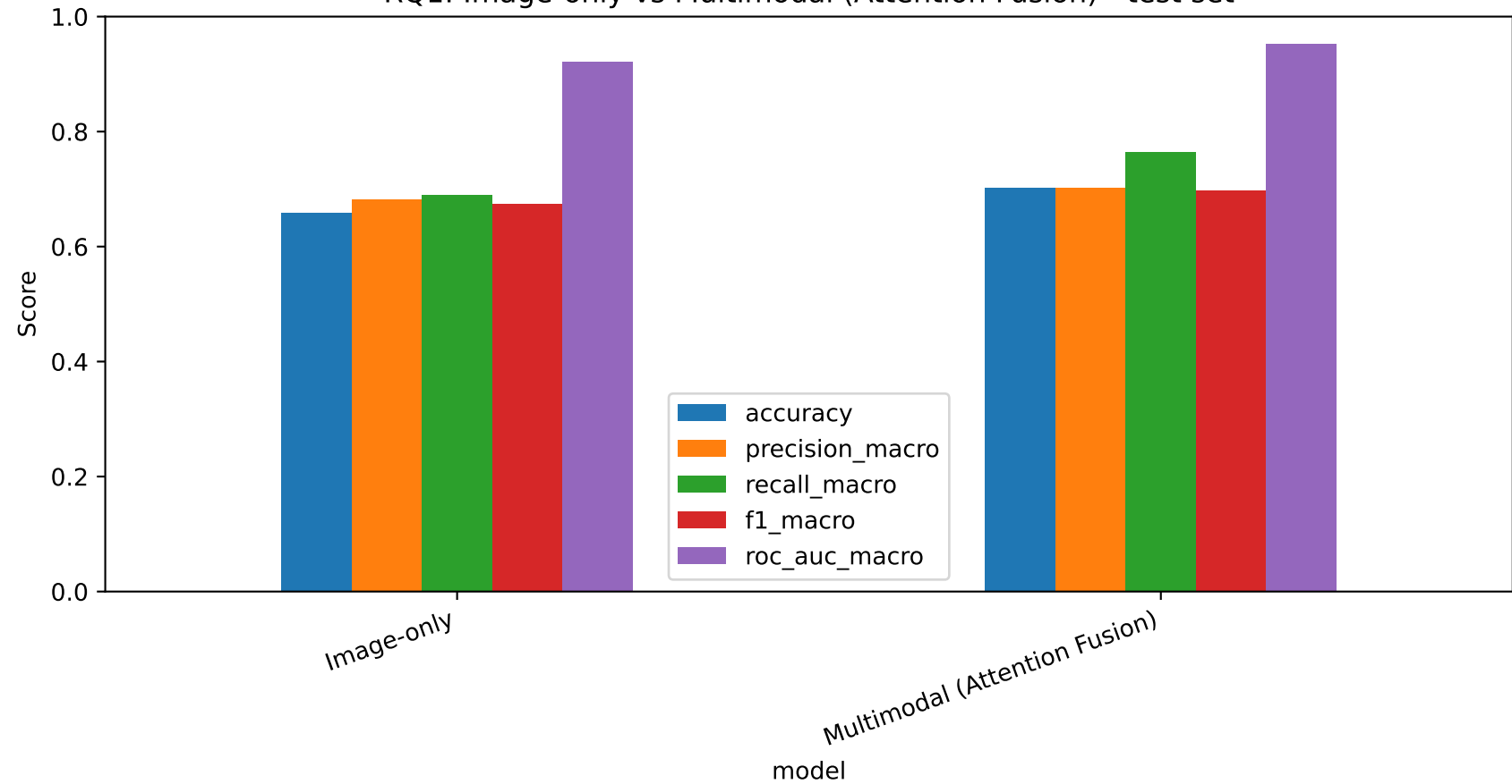
RQ1: Image-only vs Multimodal (Attention Fusion) - test set
