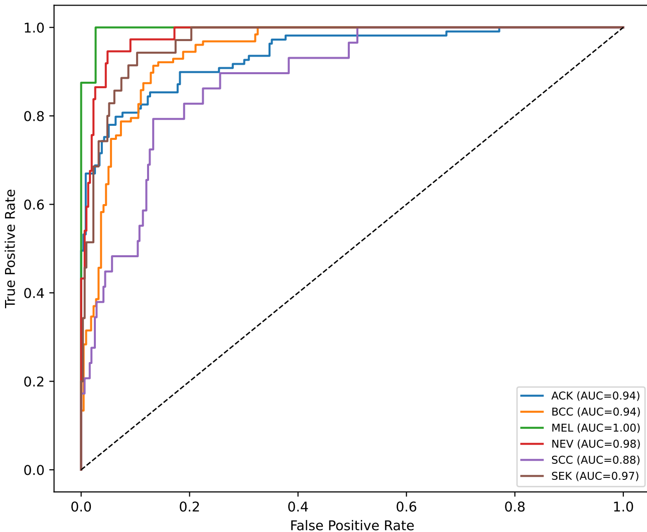
Multimodal (Attention Fusion): ROC curves (test set)
