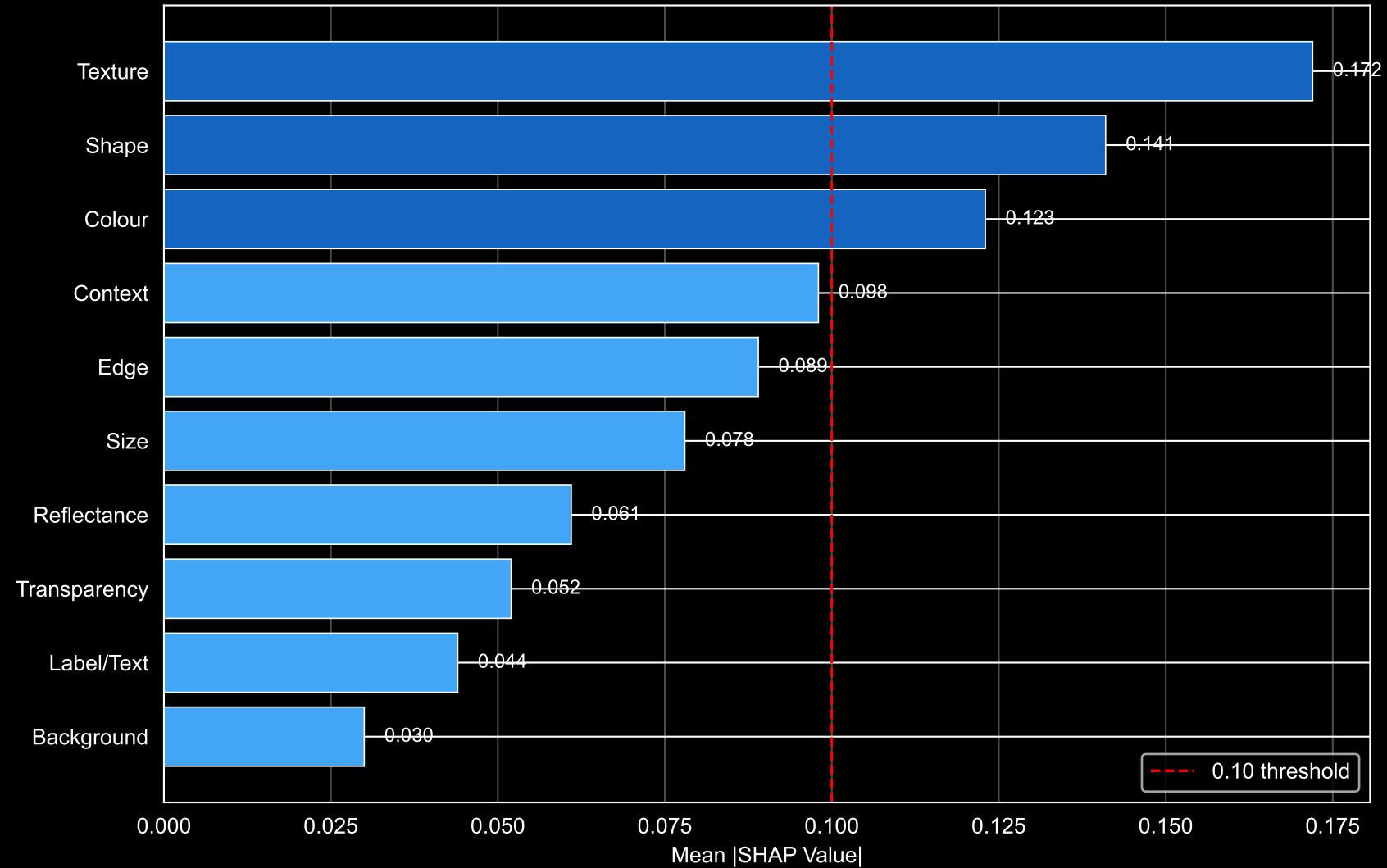
RQ2 – SHAP Feature Importance
