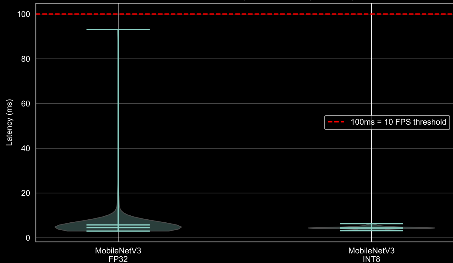
RQ5 – Inference Latency Distribution (300 runs)
