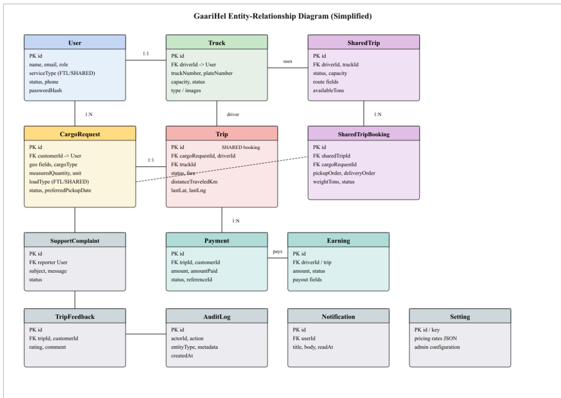
Figure A2: Entity-Relationship Diagram (ERD) of GaariHel database schema
