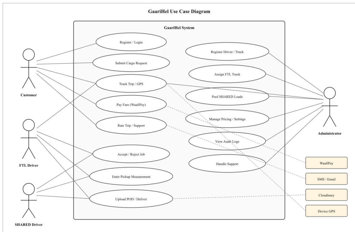
Figure A1: Use Case Diagram of GaariHel
