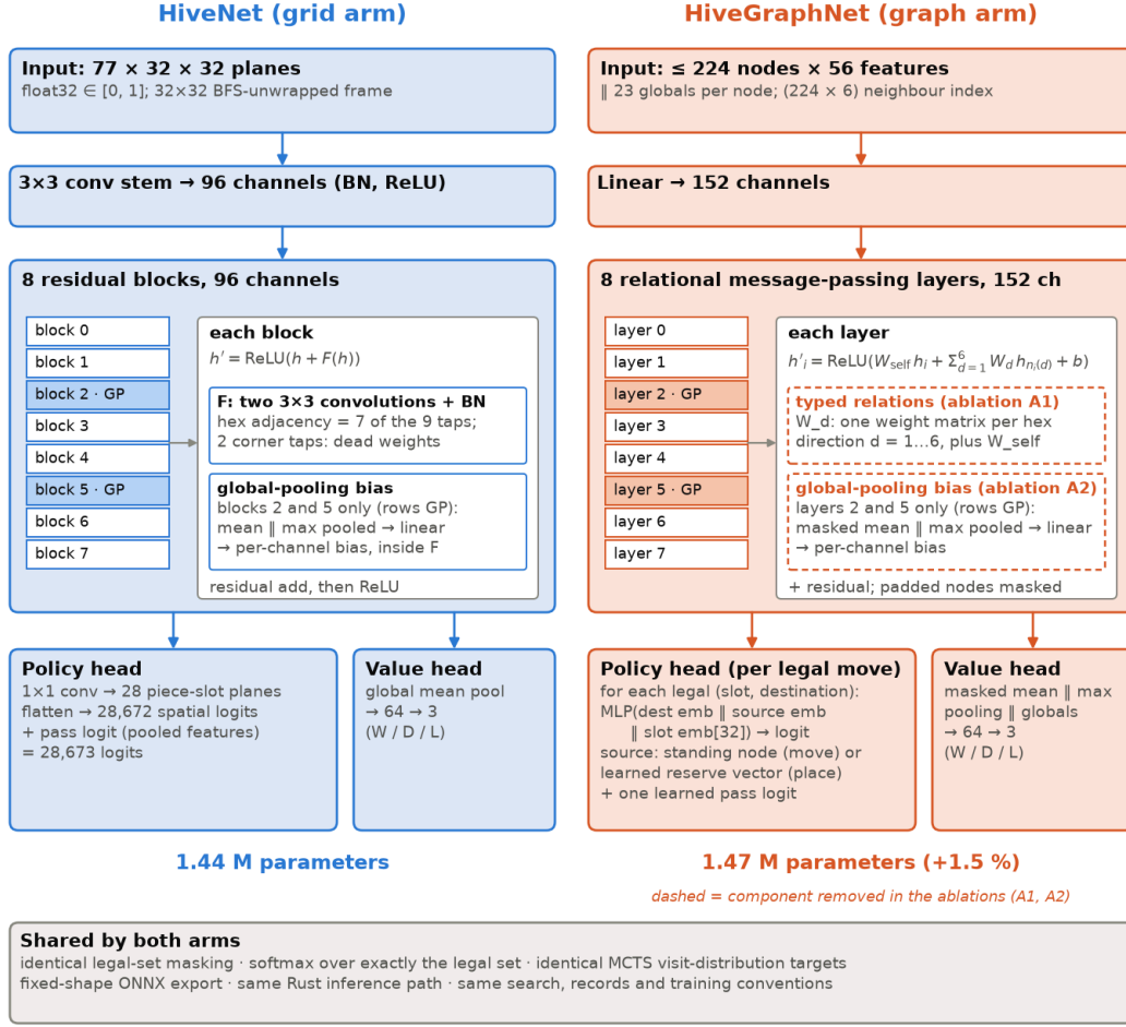
Figure 2: The two networks. Left, HiveNet (grid arm): 3 \times 3 convolutional stem, 8 residual blocks of 96 channels with a global-pooling bias in blocks 2 and 5, a flat 28,673-way policy head and a 3-way value head, 1.44 M parameters. Right, HiveGraphNet (graph arm): input layer to 152 channels, 8 relational message-passing layers with six direction-typed matrices and a global-pooling bias every third layer, a per-candidate policy scorer and a masked mean-and-max value head, 1.47 M parameters. Both feed the shared action decoder.
