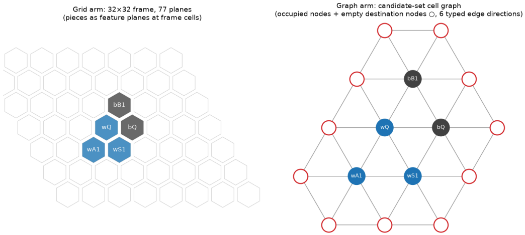
Figure 1: One position under the two encodings. Left, the grid arm’s view: the position embedded in a fixed 32 \times 32 frame of hexagonal cells, each frame cell carrying 77 feature values. Right, the graph arm’s view: the cell graph over the candidate set, in which occupied cells (filled) and empty cells adjacent to the hive (open circles) are joined by edges typed with the six hexagonal directions. Both views derive from the same engine state without loss.
