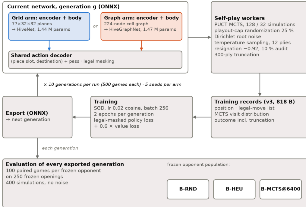
Figure 3: The generation loop shared by both arms. Self-play with Monte-Carlo tree search produces training records; the records train a network; the network is exported to ONNX and drives the next generation’s self-play; at fixed generations the exported network is evaluated against the frozen opponent population (B-RND, B-HEU, B-MCTS) on frozen openings. The grid arm and the graph arm differ only in the state encoder and the network body inside the boxes marked “network”.
