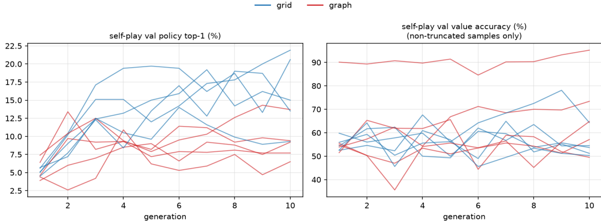
Figure 8: Training metrics by generation for the ten main-campaign runs (epoch-1 line of each generation): left, policy top-1 agreement with the MCTS visit distribution on the self-play validation split; right, value accuracy on non-truncated samples. Blue: grid arm; red: graph arm; one line per seed. Ablation runs are excluded.
