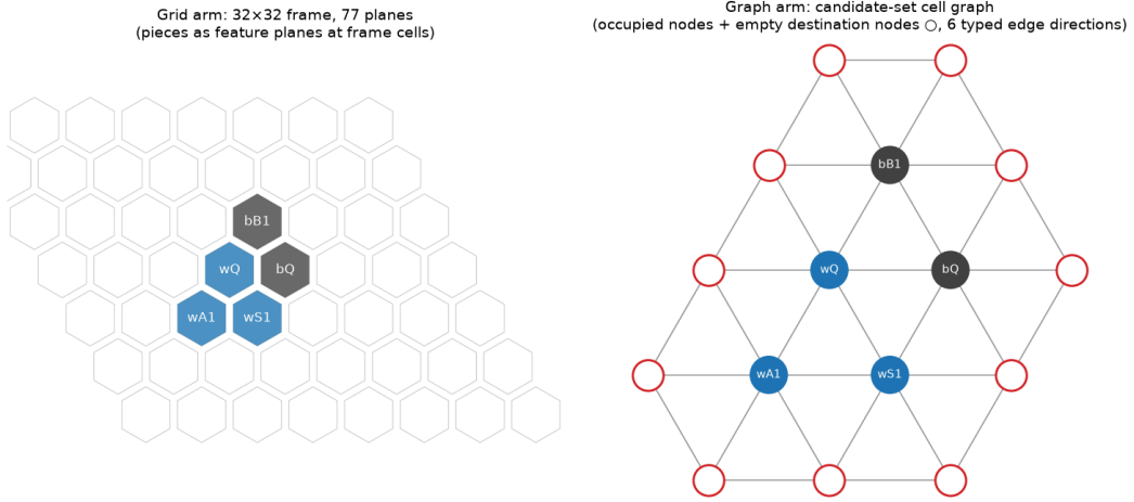
Figure 1: A five-tile Hive position under the two encodings compared in this study. Left, the grid arm’s view: the position embedded in a fixed 32×32 frame of hexagonal cells (drawn for orientation), each frame cell carrying 77 feature values, so that tiles appear as activations at frame coordinates. Right, the graph arm’s view: the cell graph over the candidate set, in which occupied cells (filled, labelled by colour and tile) and every empty cell adjacent to the hive (open circles), together the set of all legal destinations, are joined by edges typed with the six hexagonal directions. Both views derive from the same engine state without loss; only the structure offered to the network differs.
