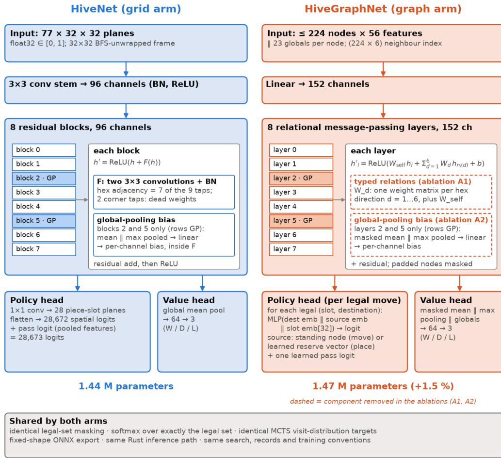
Figure 4: Block diagrams of the two networks. Left, HiveNet (grid arm): 3 \times 3 convolutional stem, 8 residual blocks of 96 channels with a global-pooling bias in blocks 2 and 5, a flat 28,673-way policy head and a 3-way value head, 1.44 M parameters in total. Right, HiveGraphNet (graph arm): input linear layer to 152 channels, 8 relational message-passing layers with six direction-typed matrices and a global-pooling bias every third layer, a per-candidate policy scorer over destination, source and slot embeddings, and a masked mean||max value head, 1.47 M parameters in total. Both networks feed the shared action decoder; only the encoder and the body differ.
