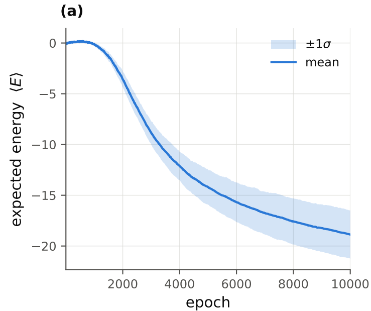
RBM learning as thermodynamic relaxation (2x2 BAS, n_v = n_h = 4 , T = 1 , CD-1, 50 seeds)
