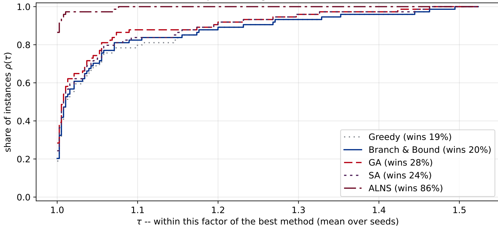
Performance profile, Augerat A/B/P (74 instances)
