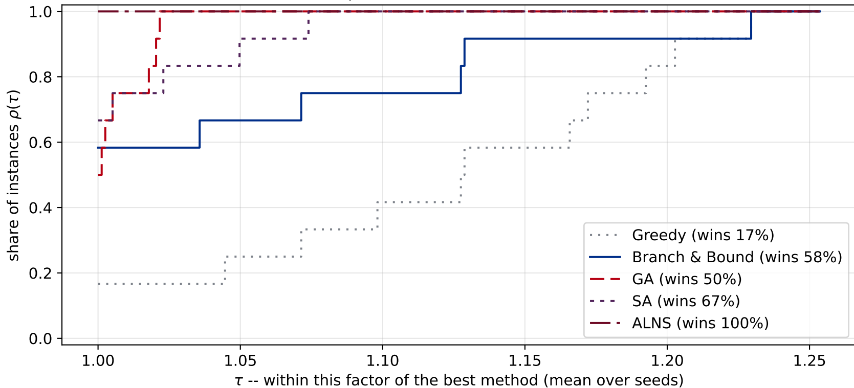
Performance profile, Pontianak suite (12 instances)
