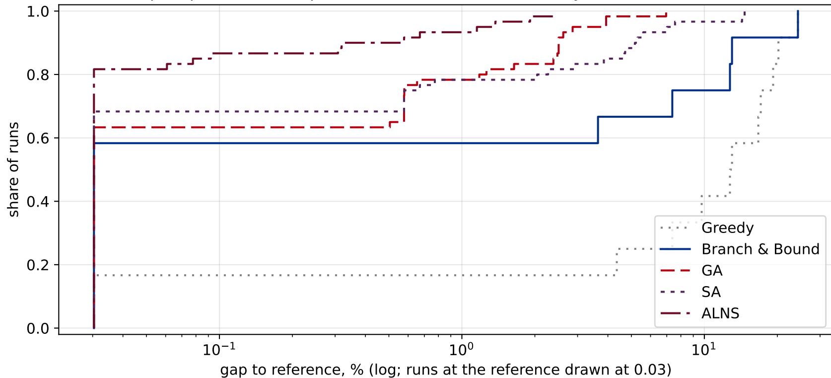
Gap to proven B&B optimum, else best found, every run, Pontianak suite
